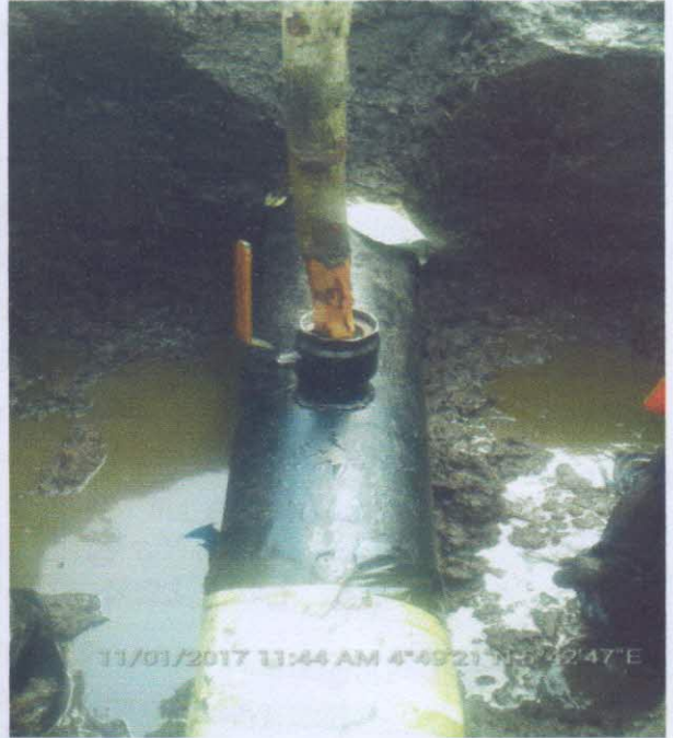
FIG 2: Spill point on excavation
